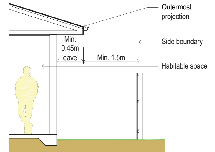
Diagram 2.3 – Boundary setbacks for lots under 600m 2
