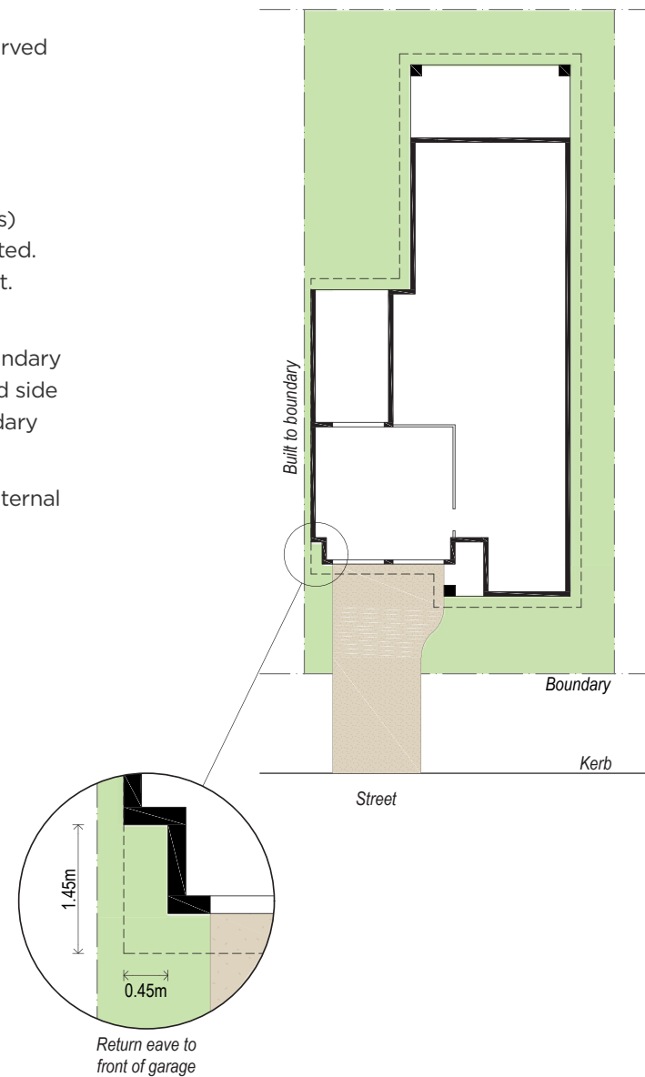
Diagram 5.1 – Roofing
